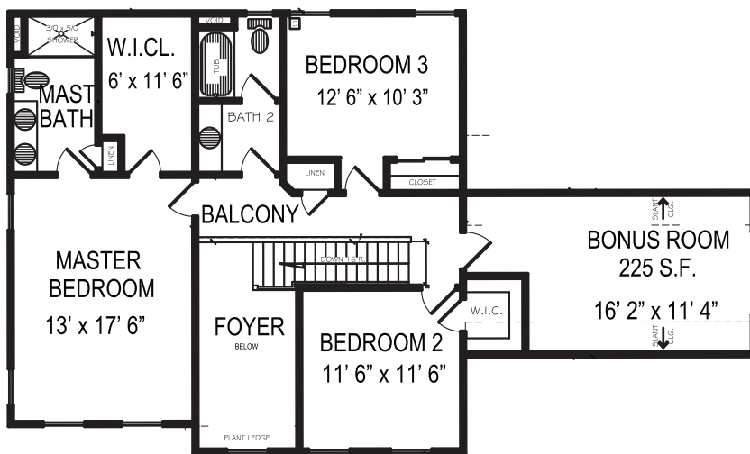
SECOND FLOOR PLAN 1182 S.F. INCLUDING 225 S.F. BONUS RM.
